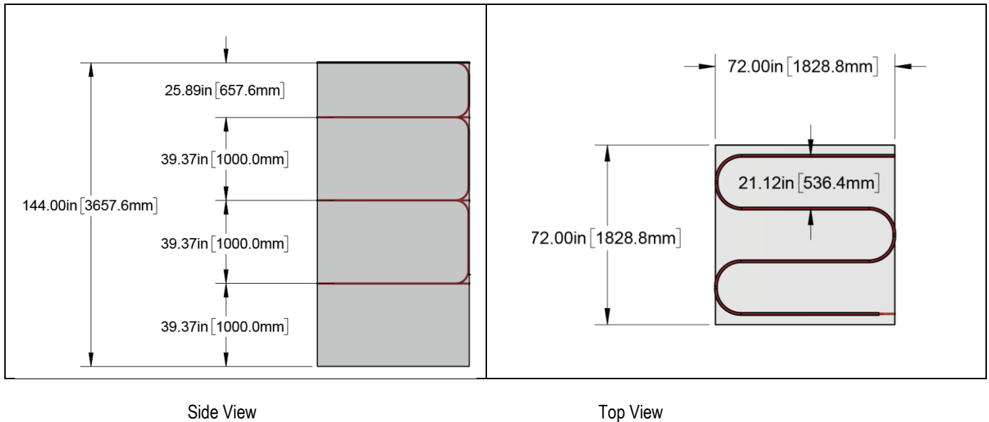
Figure 16 – Tubing Configuration Guideline (Side View and Top View)
