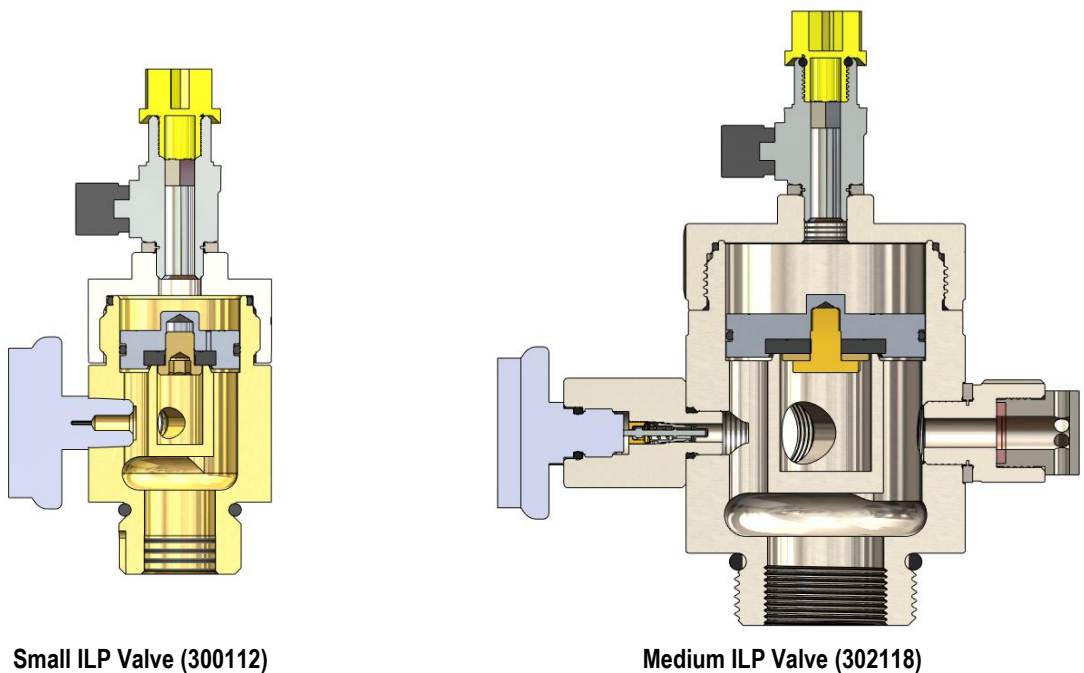
Figure 3 – Cylinder Valves
