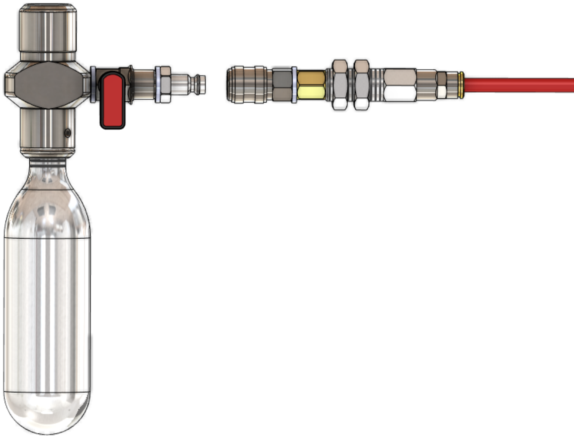
Figure 18 – Firetrace Nitrogen Charge Kit 600213
