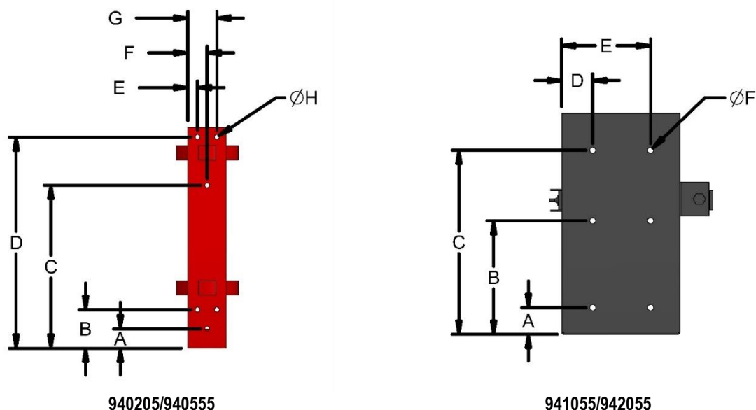
Figure 2 – Cylinder Mounting Bracket Bolt Pattern
