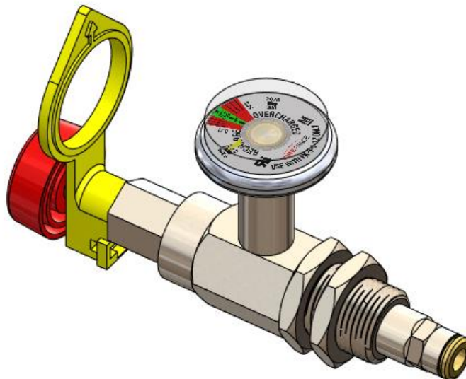
Figure 5 – Manual Release
