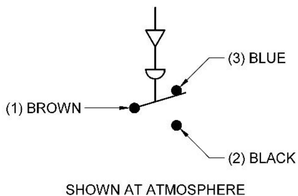
Figure 10 –Pressure Switch Wiring Schematic
